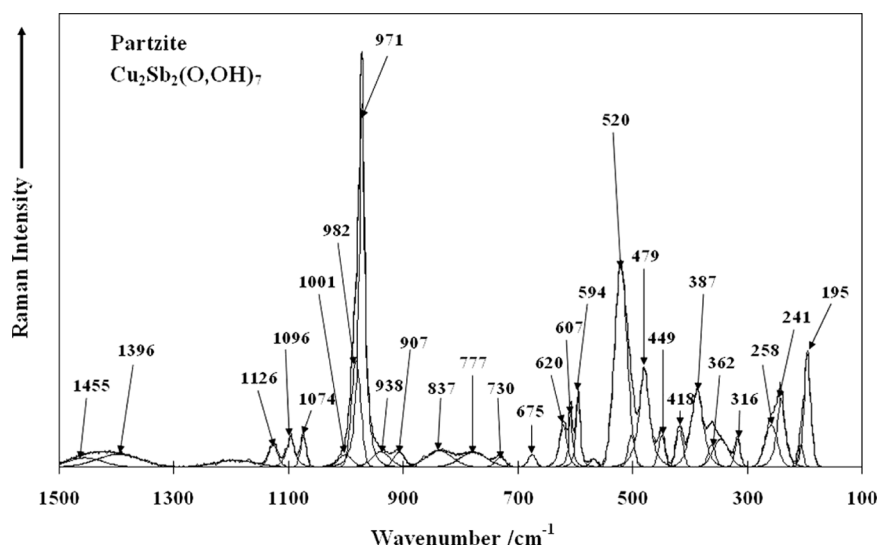
FIGURE 1 Raman spectrum of partzite in the 100 to 1500 \text{cm}^{-1} region.
