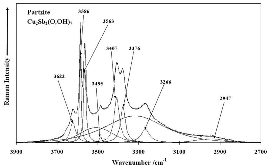
FIGURE 2 Raman spectrum of partzite in the 2700 to 3900 \text{cm}^{-1} region.
